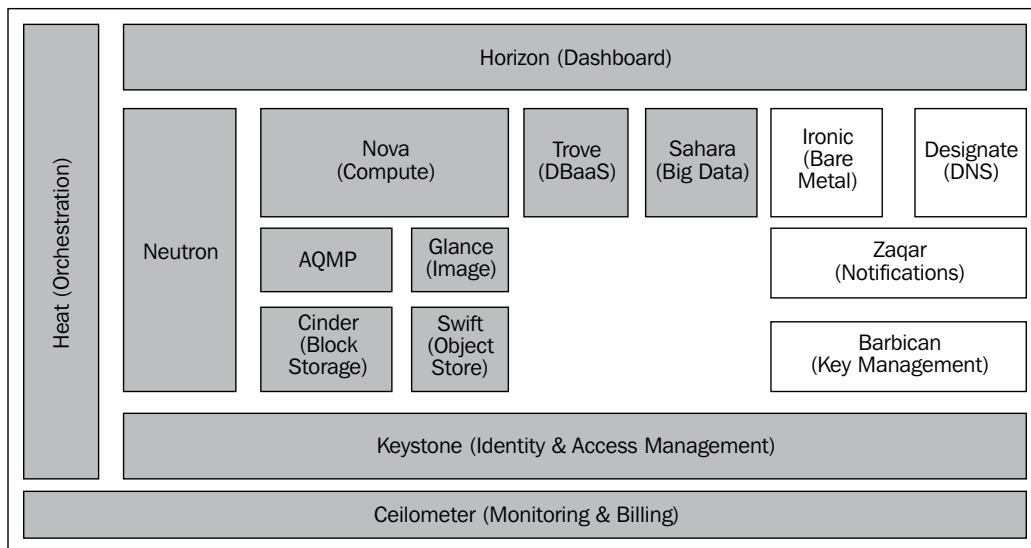
An OpenStack block diagram
