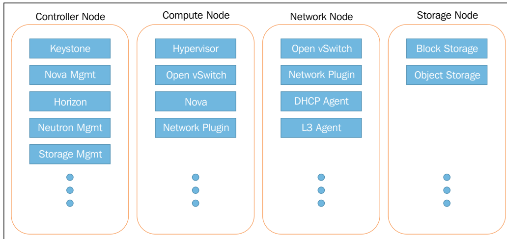
The OpenStack service layout
